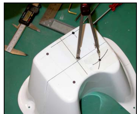
(below) Use a pair of compasses to mark the 78mm and 44mm arcs for positioning the 2nd hole.
