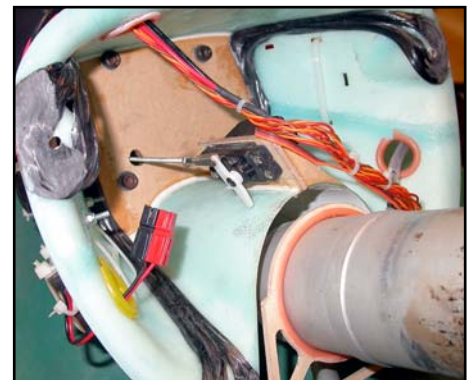
Milled bulkhead around the front of the mini-pipe is also protected from heat with a split silicone tube, that is supplied in the kit.
