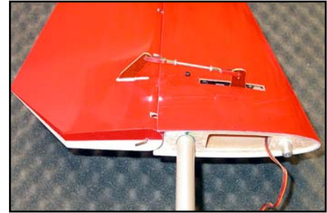
Shows stab retaining bolt, 20mm aluminium spar, anti-rotation pin, C-ARF servo arm and linkage. Note the elevator horn is located slightly differently on production kits.
