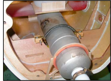
(above) Mini-pipe mounted with the milled ply front bulkhead and a brass strap/spring at the back.
