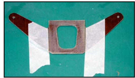
(above) Rudder horn roughed up with coarse sandpaper.
