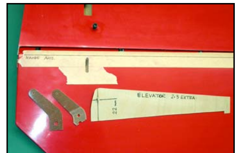
(above) Shows horn alignment template made from scrap ply, and both standard and modified C-ARF control surface horns.
