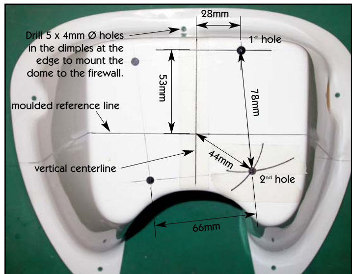
(above) Dimensions for mounting holes for DA-50 motor stand-offs.
