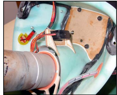
2 views inside the back of the motor dome, showing the carbon tow strengthening, and the throttle servo mount from scrap 3mm plywood. Note the cutouts in the motordome for all cables are protected with split silicone tube (or rubber grommets).
