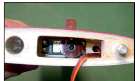
Elevator servo installed, with C-ARF servo horn. Drill an 8mm Ø hole in the rib about 15mm in front of servo for cable and connector.
