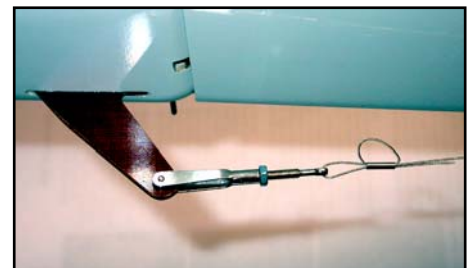
(below) Pass rudder cable thru' crimping tubes 2 times for safety.
